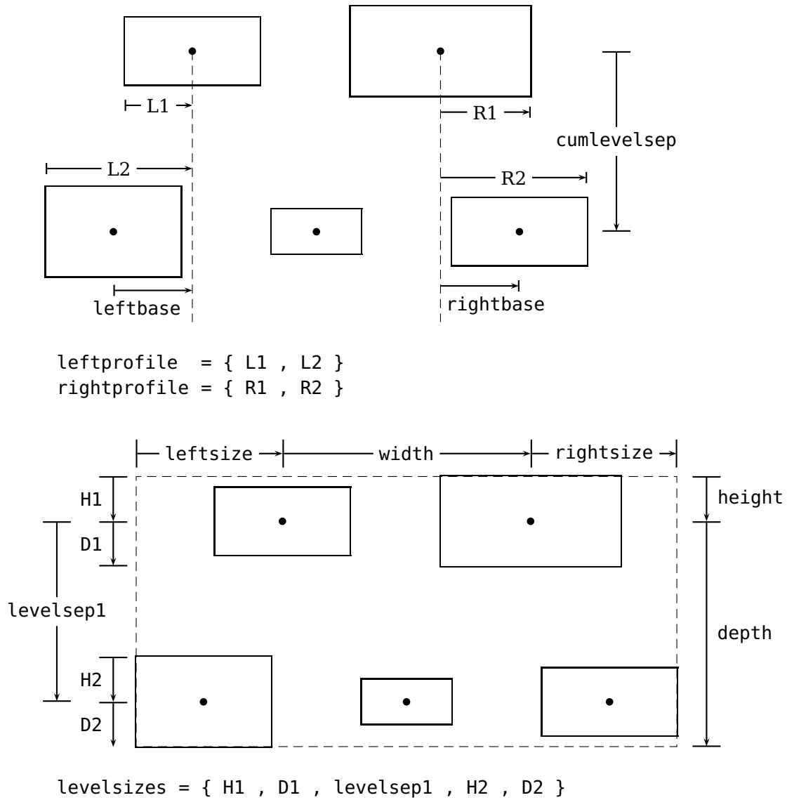
Figure 2: Tree data
